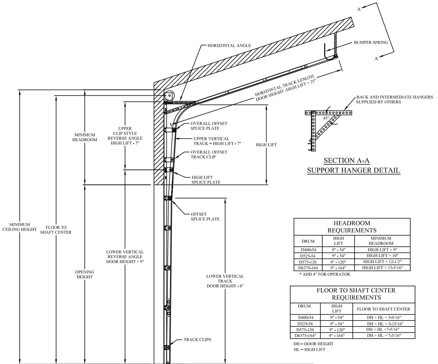
HIGH LIFT ANGLE MOUNT TRACK SET DETAIL
