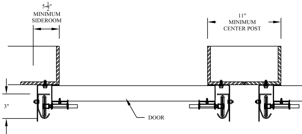
COMMERCIAL TAPERED REVERSE ANGLE MOUNT TO STEEL JAMB DETAIL
