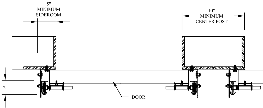
COMMERCIAL REVERSE ANGLE MOUNT TO STEEL JAMB DETAIL
