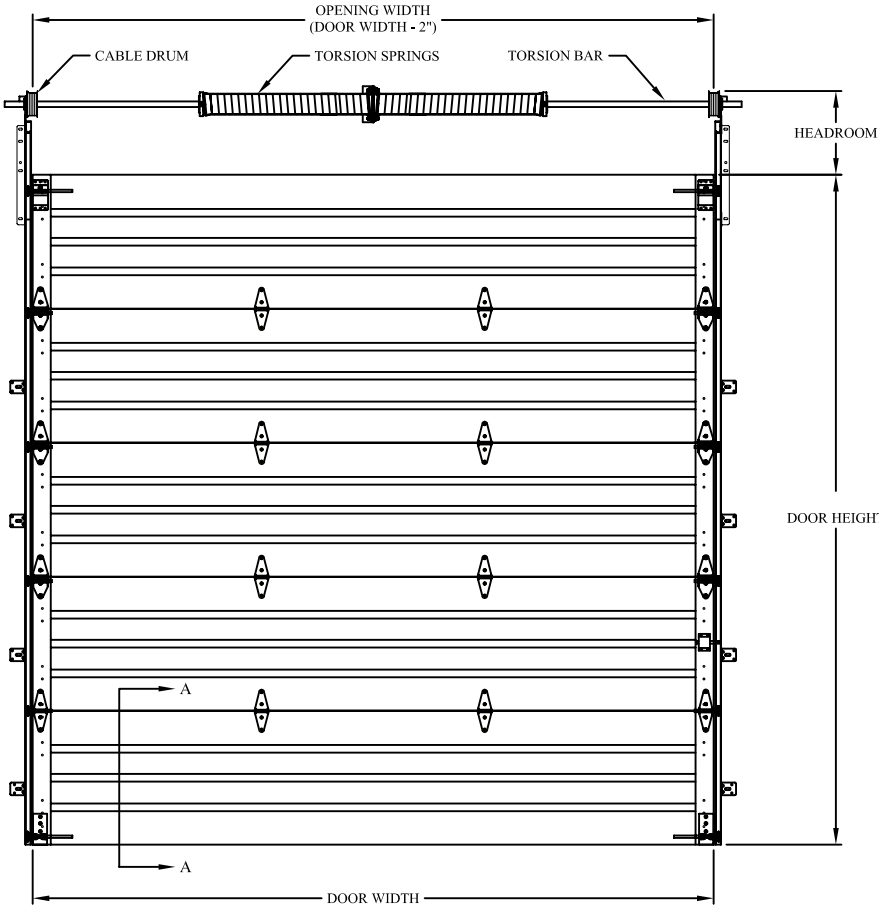
INTERIOR ELEVATION
