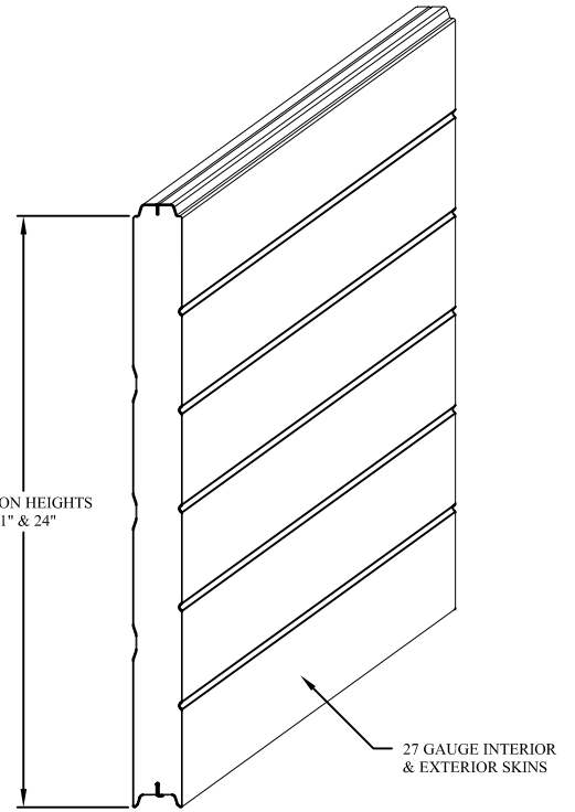
ISOMETRIC PROFILE
